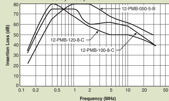
12-PMB-050;-100;-120
